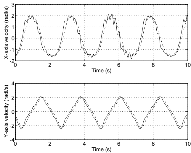
Figure 7.37: Measured tracking velocity for target on turntable revolving at 4.2 rad/s, showing axis velocity (solid) and estimated target velocity (dashed). Note that the Y-axis (tilt) velocity is somewhat triangular — this is due to the 1/S_6 term in the tilt kinematics given by (6.6). This data was logged by RTVL.
