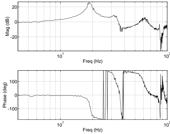
Figure 8.6: Measured frequency response function 1/(j\omega)^2\ddot{X}_{cam}/\Theta_m which includes arm structure and transmission dynamics. The first resonance is at 19Hz. Good coherence was obtained above 4Hz.
