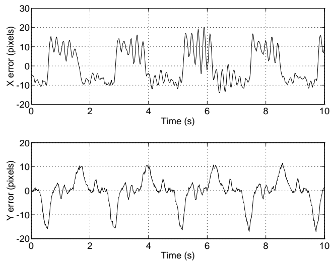
Figure 7.36: Measured tracking performance, centroid error, for target on turntable revolving at 4.2 rad/s. This data was logged by RTVL.
