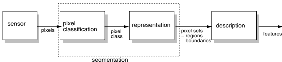
Figure 4.1: Steps involved in scene interpretation
