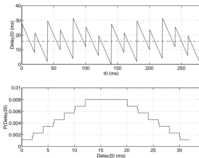
Figure 6.25: Analysis of sampling time delay \Delta_{20} for the case where T_1 = 20 ms and T_2 = 14 ms. Top shows variation in delay versus sampling time (mean of 16 ms shown dashed), while bottom shows probability distribution.
