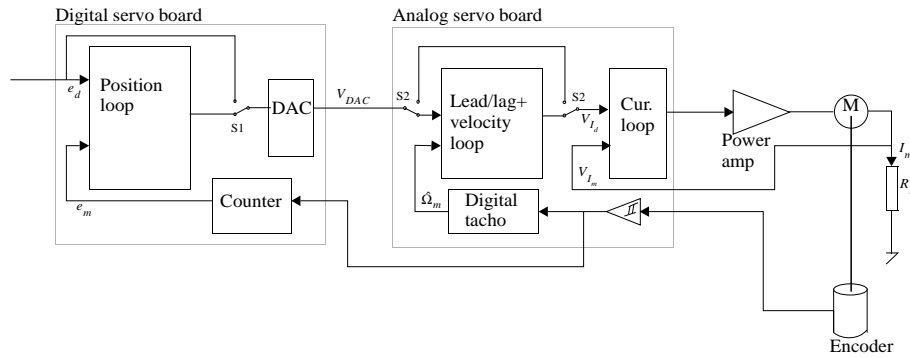
Figure 2.22: Unimodulation servo position control mode. The switch S2 routes the output of the DAC to the lead compensator and velocity loop.
