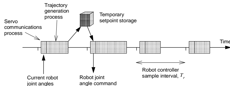
Figure 6.4: Timing of ARCL setpoint generator and servo communication processes.
