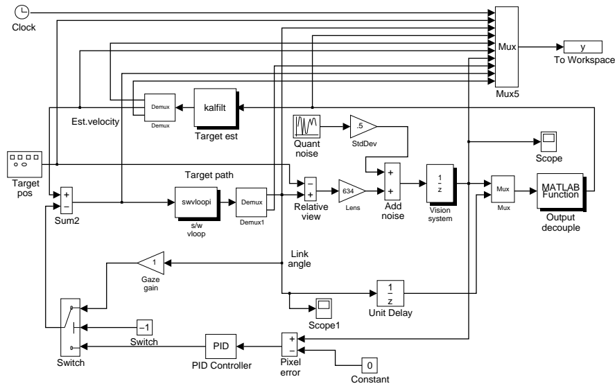
Figure 7.33: SIMULINK model FFVSERVO: feedforward fixation controller.
